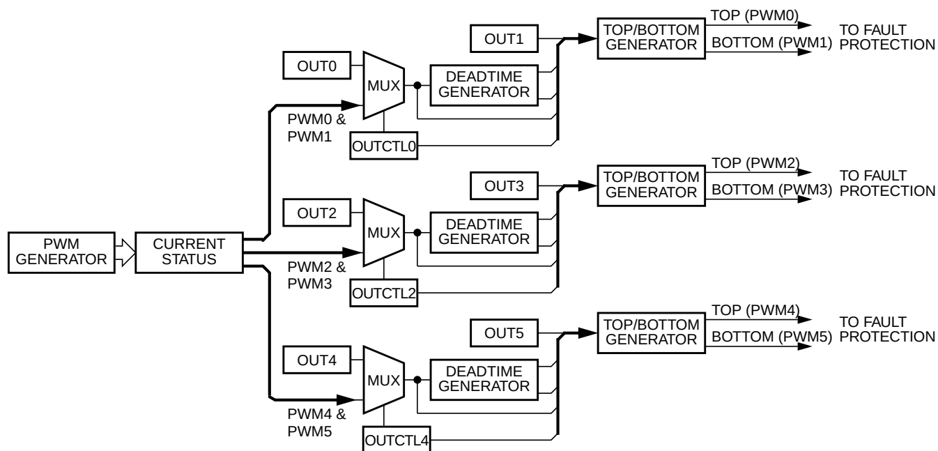
Figure 11-49. Deadtime Generators
