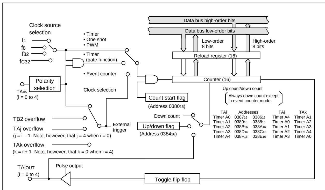
Fig.FB-3 Block diagram of timer A
