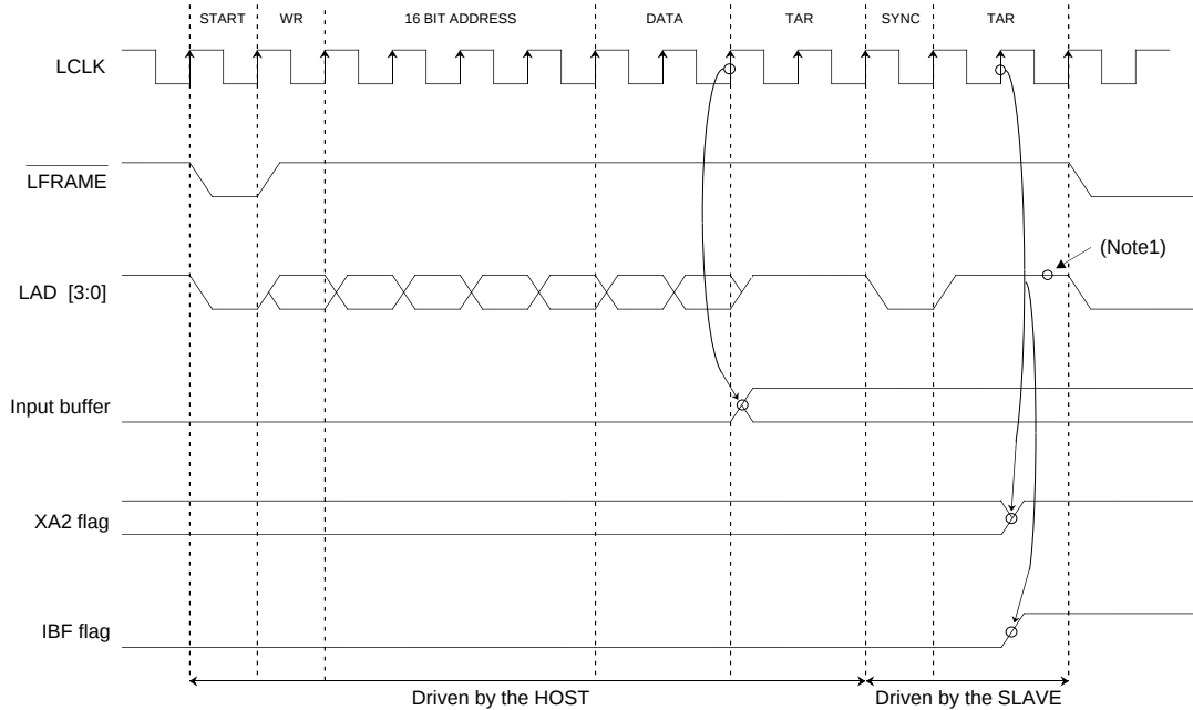
Fig.GF-7 Data and Command write timing figure
