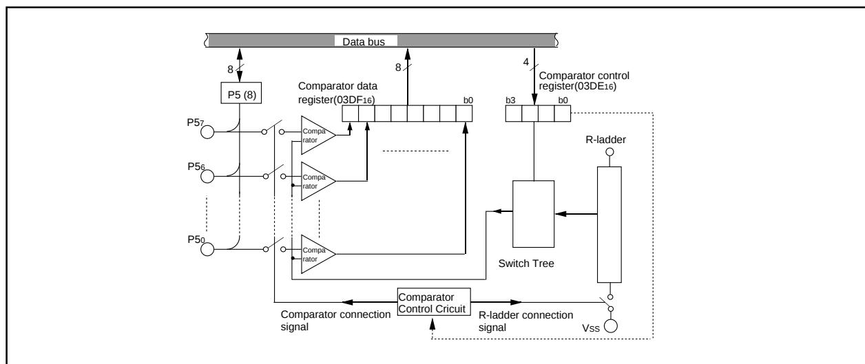
Fig.JC-1 Comparator circuit
