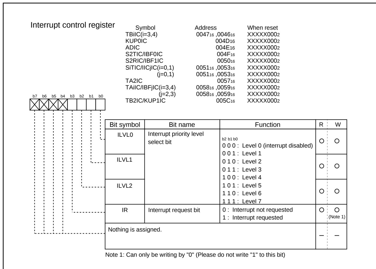
Fig.DD-3 Interrupt control registers(1)
