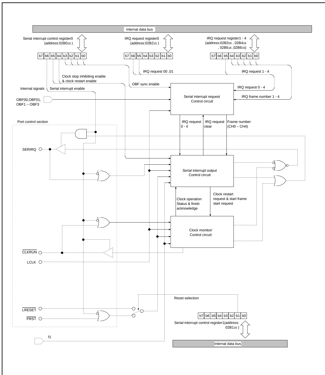
Fig.SI-1 Serial interrupt block chart
