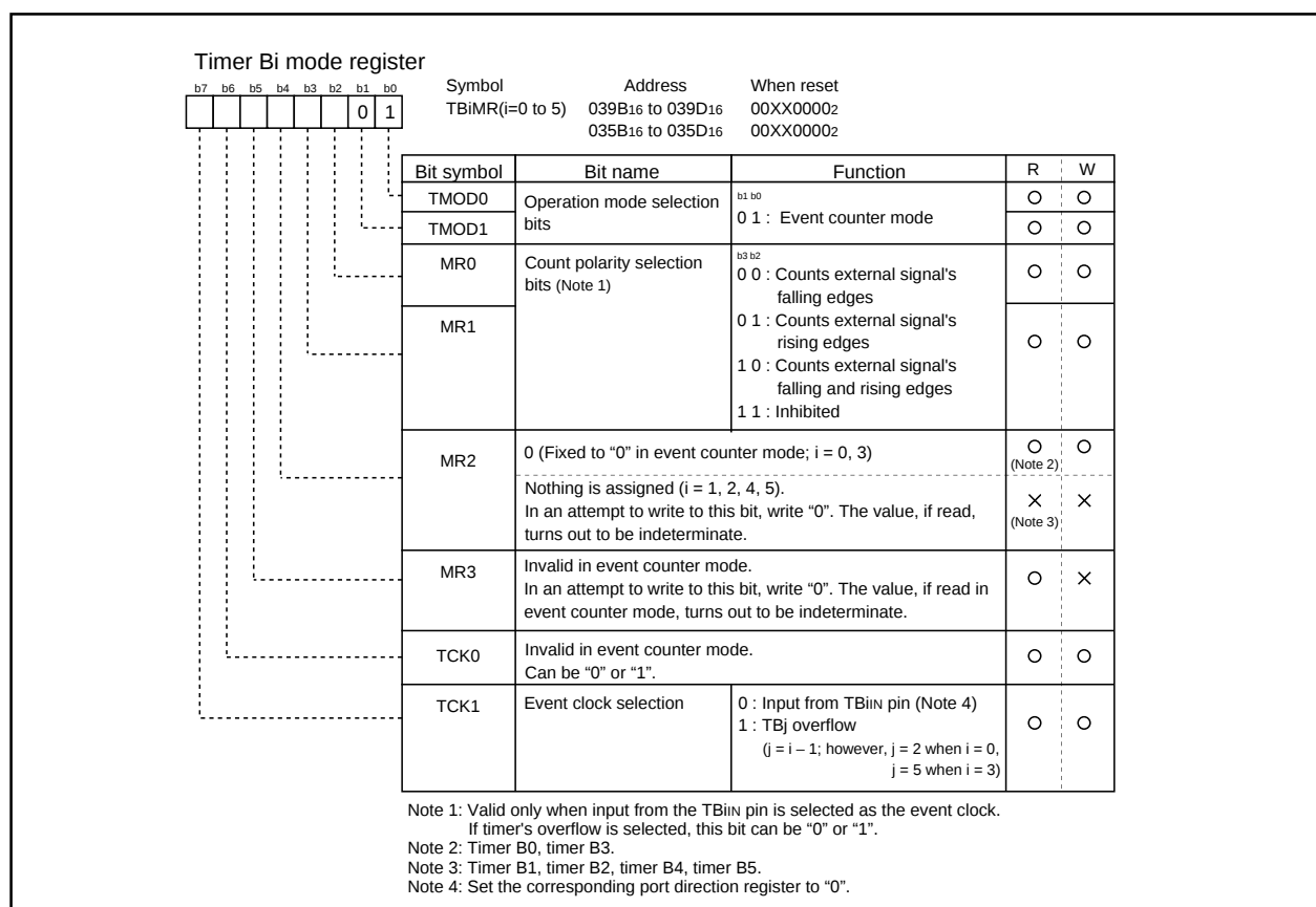
Fig.FB-18 Timer Bi mode register in event counter mode
