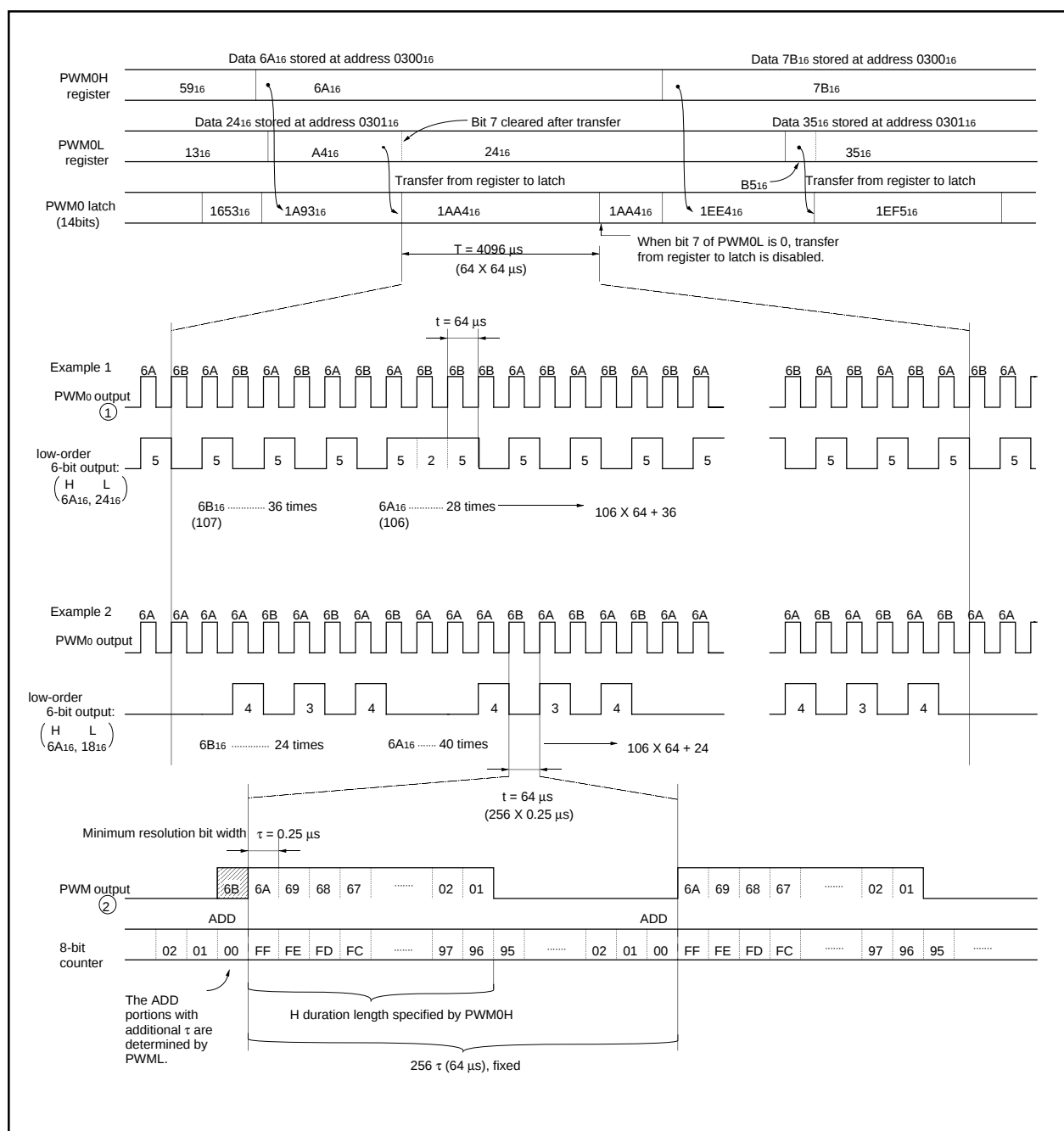
Fig.LA-3 14-bit PWM timing (PWM0)
