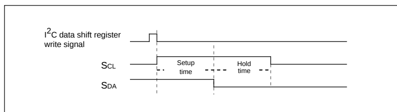
Fig.GC-17 Start condition generation timing diagram
