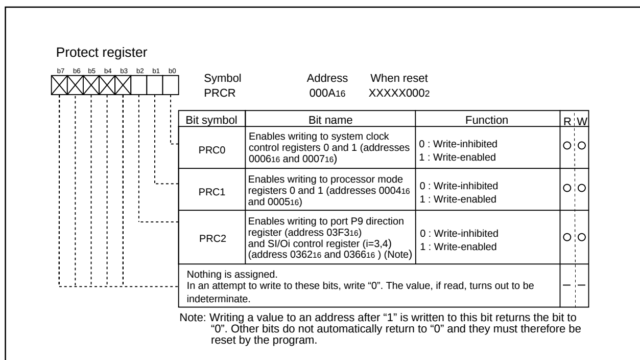
Fig.WA-6 Protect register
