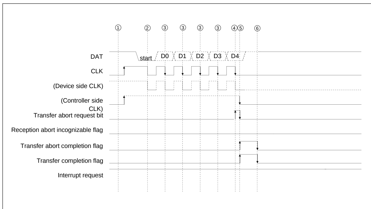
Fig.GK-11 Transfer abort operation timing ( reception)
