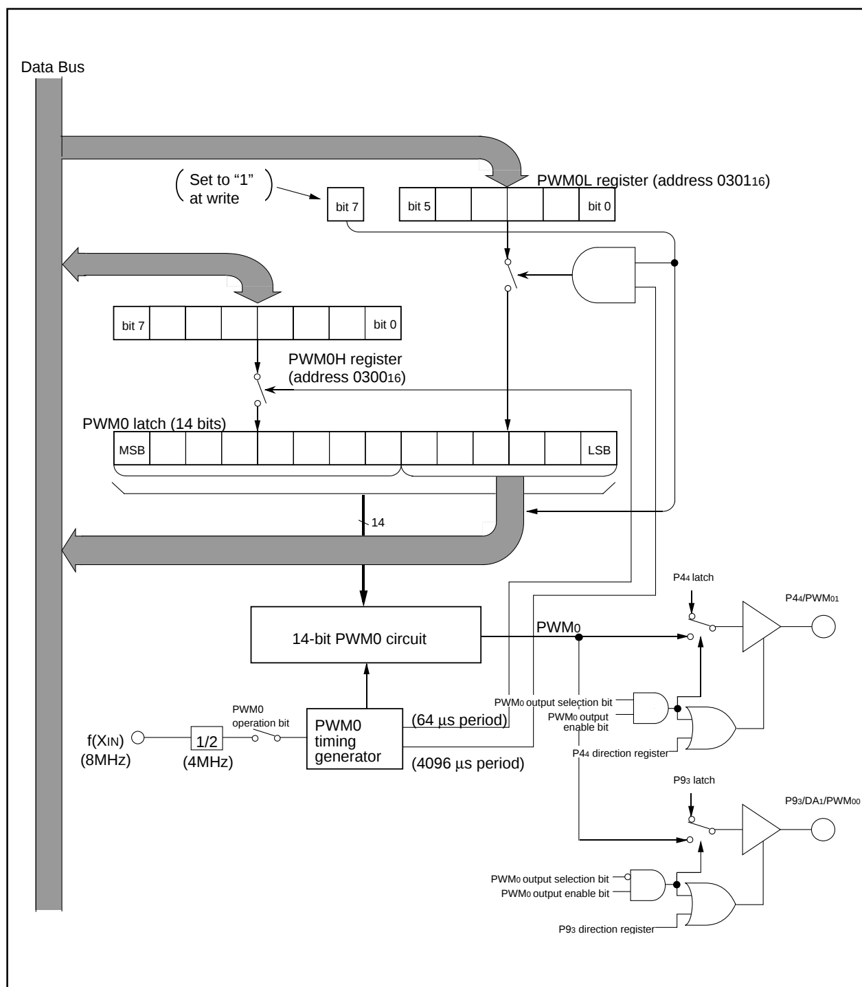
Fig.LA-1 PWM block diagram(PWM0)
