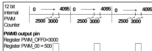
Figure 9: PWM operation
