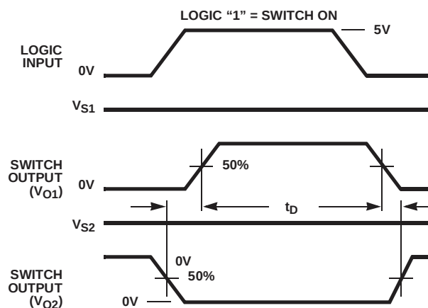
FIGURE 2. BREAK-BEFORE MAKE TEST CIRCUIT AND MEASUREMENT POINTS (DG301A, DG303A)
