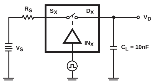
FIGURE 1. CHARGE INJECTION TEST CIRCUIT AND MEASUREMENT POINTS
