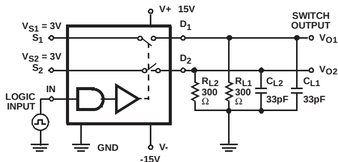
FIGURE 2. BREAK-BEFORE MAKE TEST CIRCUIT AND MEASUREMENT POINTS (DG301A, DG303A)
