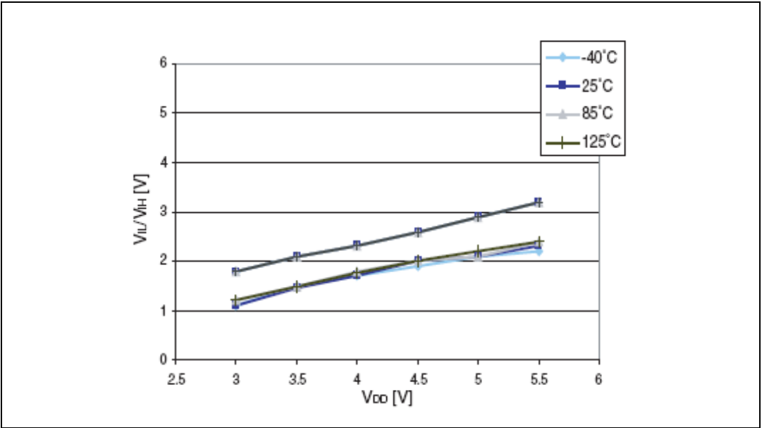
Figure 17. Typical V_{IL} and V_{IH} vs V_{DD} @ 4 temperatures
