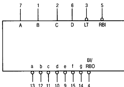
LOGIC SYMBOL
