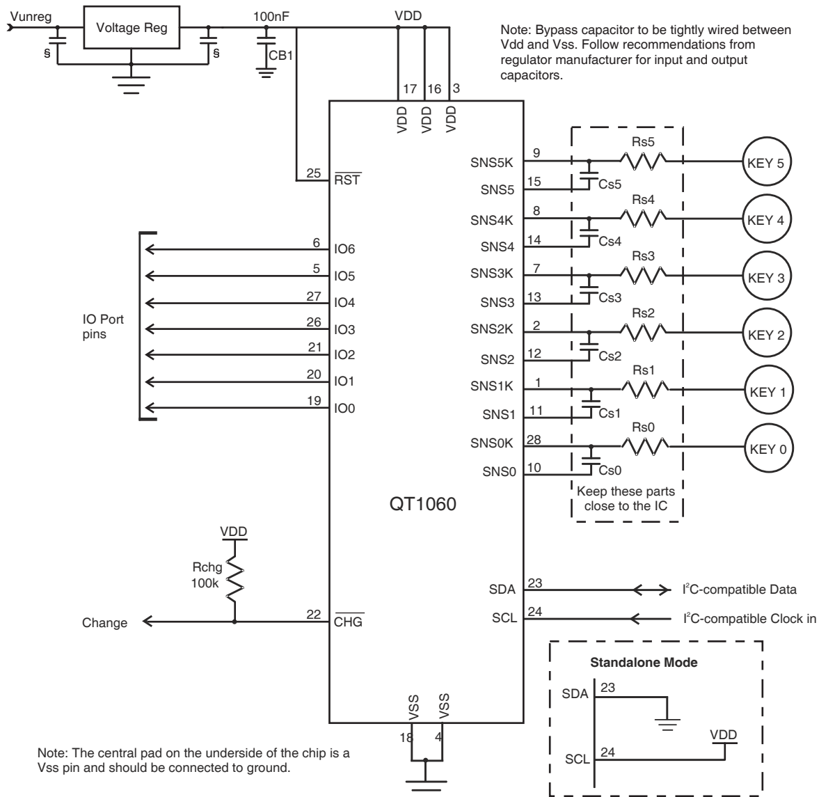
Figure 1-1. Typical Circuit
