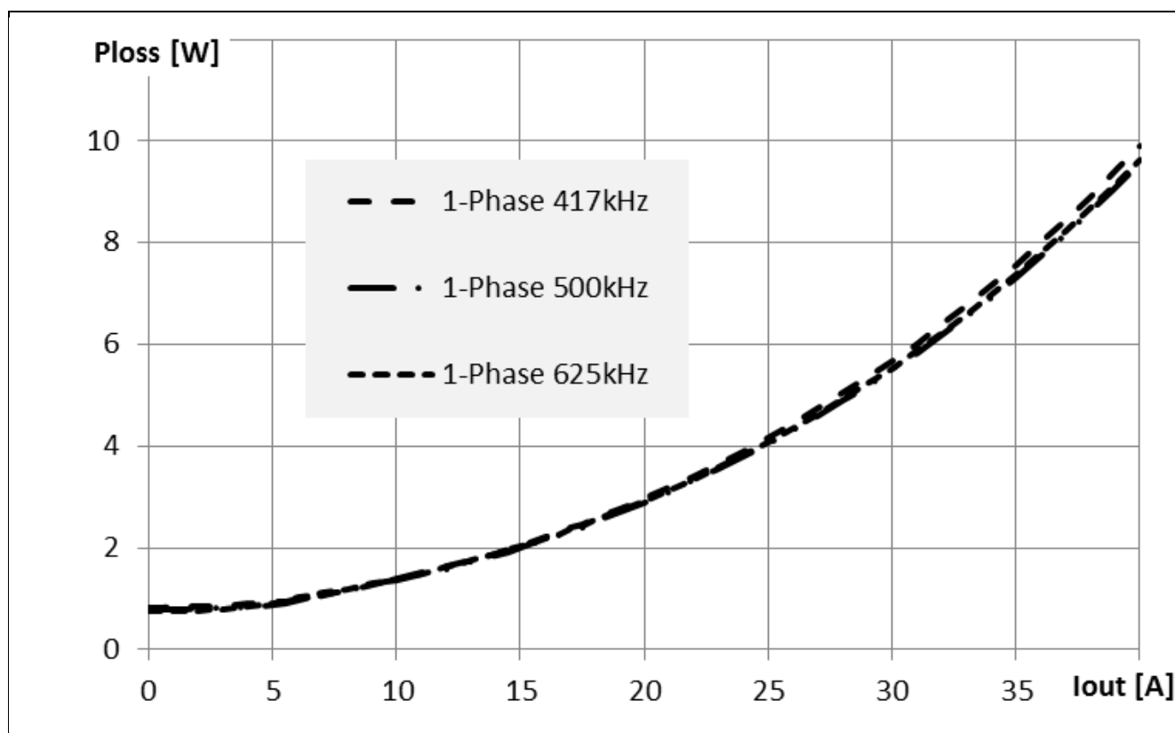
Figure 17 Power Loss at V_{IN} = 12\text{ V} , V_{CC} = PV_{CC} = 5\text{ V} , Single Phase, V_{OUT} = 1.2\text{ V}
