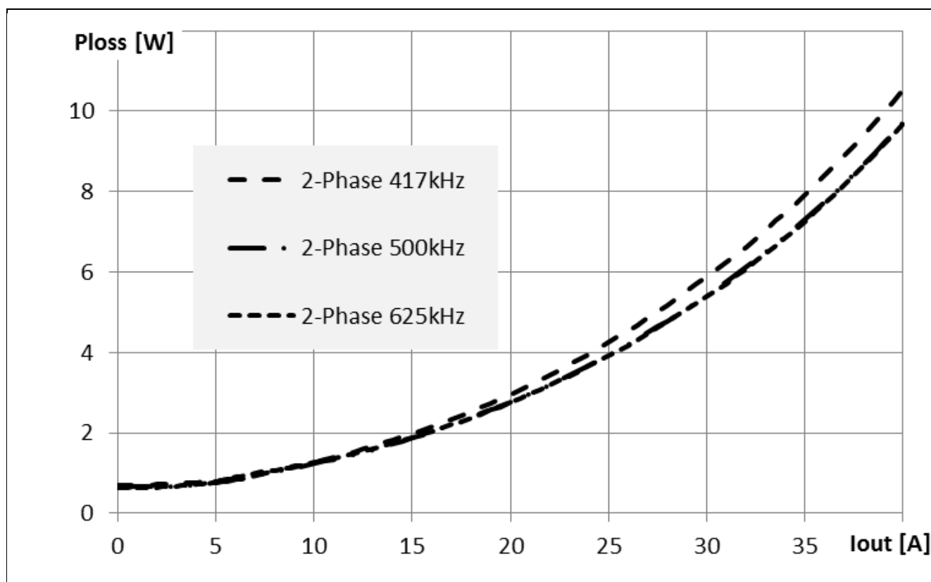
Figure 18 Power Loss at V_{IN} = 12\text{ V} , V_{CC} = PV_{CC} = 5\text{ V} , Dual Phase, V_{OUT} = 1.2\text{ V}
