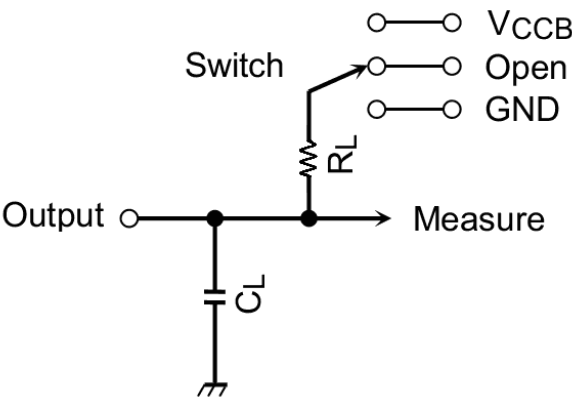
Fig. 12.1 AC Test Circuit
