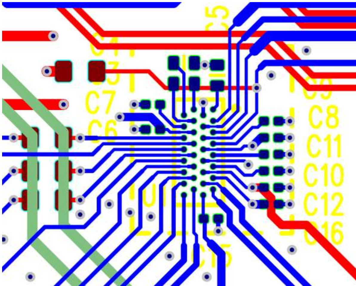
Figure 45: DA7218 example layout
