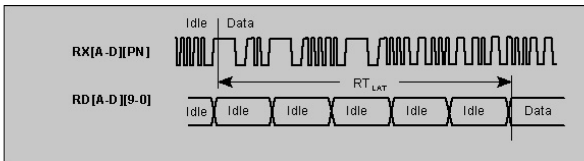
FIGURE 6-4. RECEIVER LATENCY
