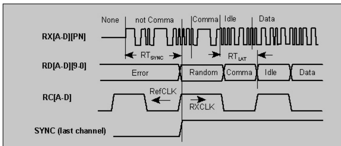
FIGURE 6-5. BYTE SYNCHRONIZATION
