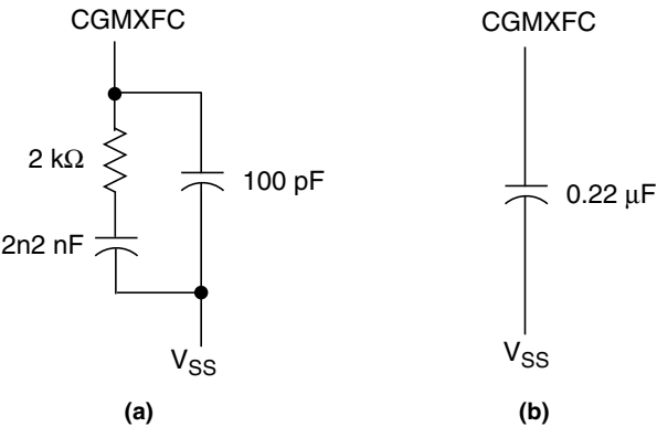
Figure 5-10. PLL Filter
