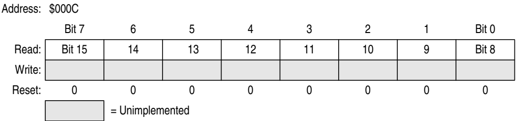
Figure 8-5. TIM Counter Registers High (TCNTH)
