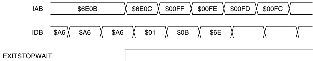
Figure 6-16. Wait Recovery from Interrupt or Break
