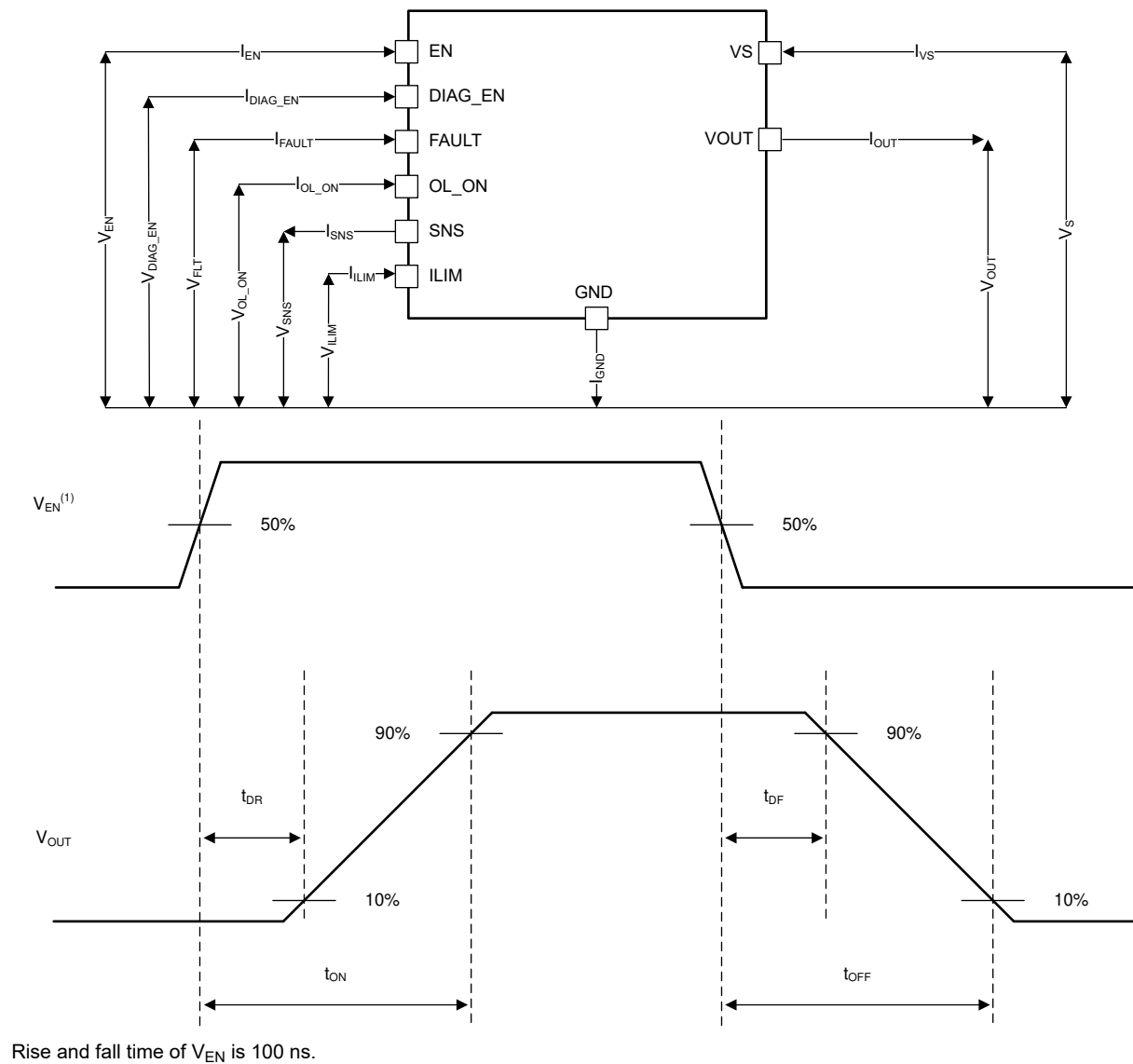
Figure 8-2. Switching Characteristics Definitions
