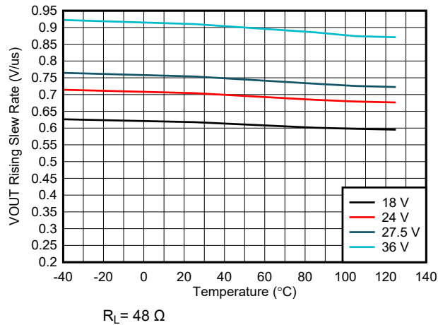
Figure 7-9. VOUT Rising Slew Rate ( SR_R ) vs Temperature vs VS Voltage
