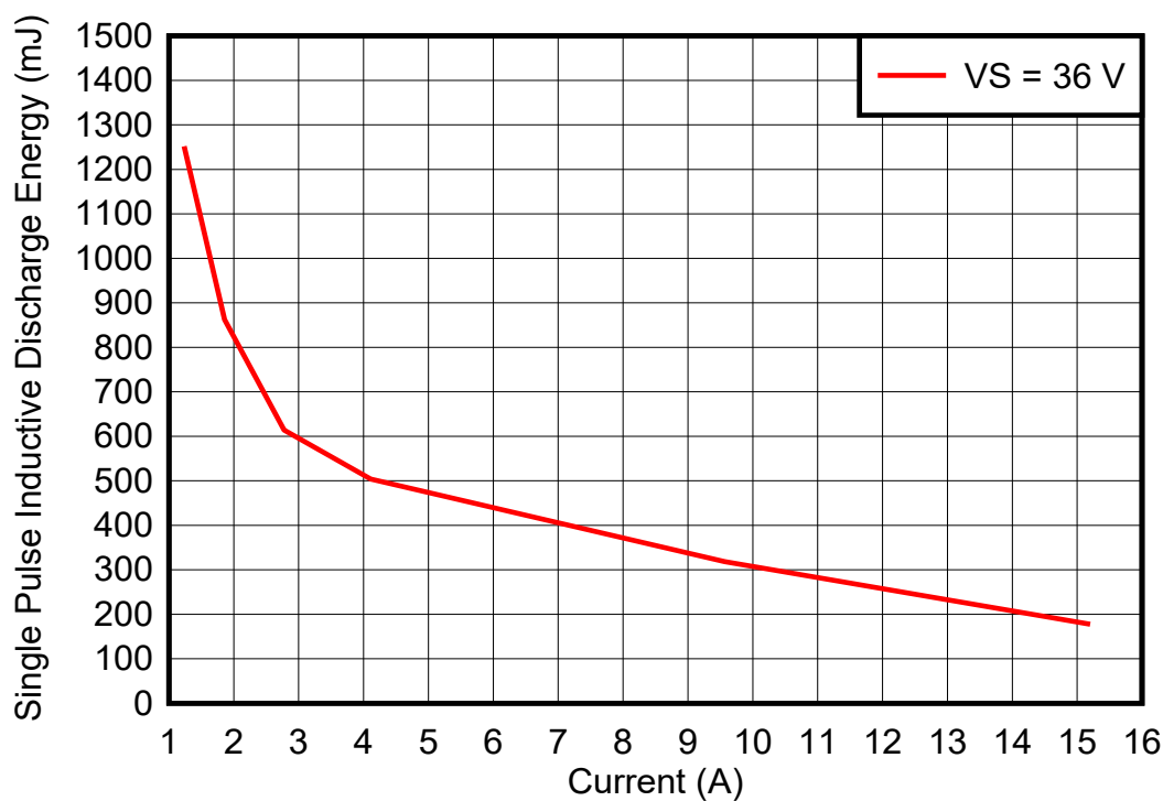
Figure 9-14. TPS281C30 Inductive Load Discharge Energy Capability at 125°C
