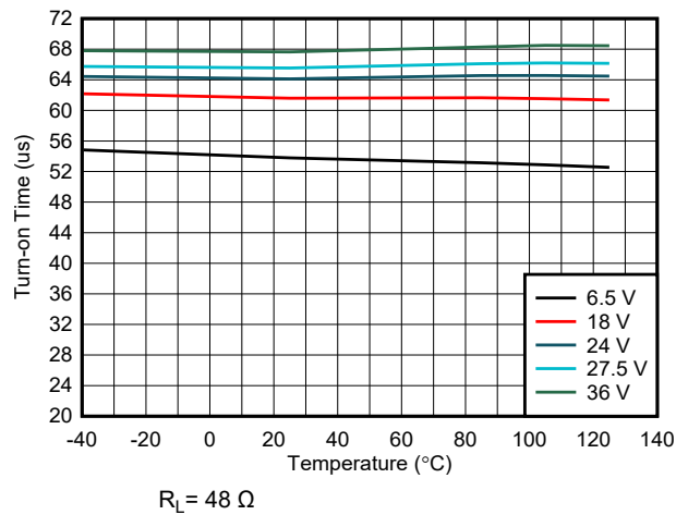
Figure 7-7. Turn-on Time ( t_{ON} ) vs Temperature vs VS Voltage
