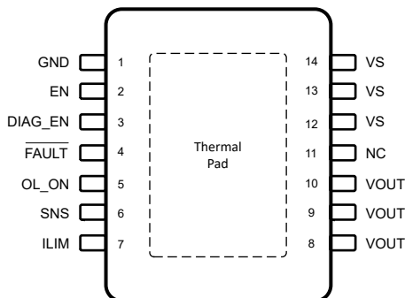
Figure 6-1. PWP Package, 14-Pin HTSSOP (Top View)
