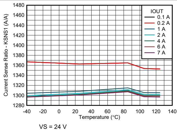
Figure 7-11. Current Sense Ratio ( KSNS_1 ) vs Temperature vs Load Current
