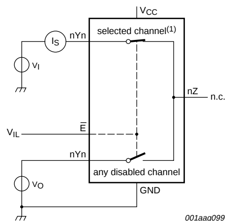
(1) Channel is selected by S0 and S1. Fig 7. Test circuit for measuring ON-state leakage current
