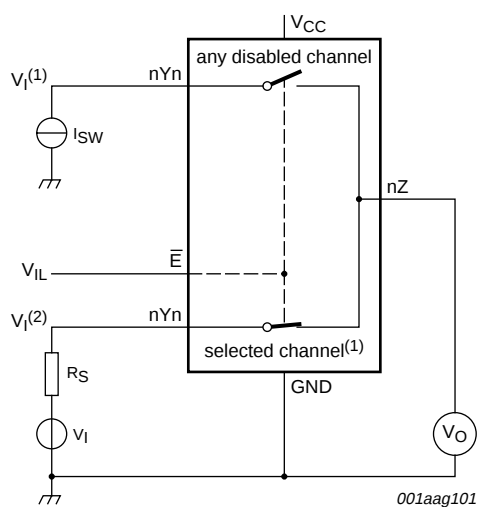
(1) Channel is selected by S0 and S1. V_I^{(1)} < \text{GND} or V_I^{(1)} > V_{CC} . \text{GND} < V_I^{(2)} < V_{CC} . Fig 9. Test circuit for injection current coupling
