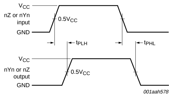
Fig 10. Input (nZ, nYn) to output (nYn, nZ) propagation delays
