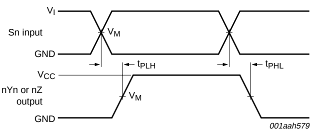
Fig 11. Input (Sn) to output (nYn, nZ) propagation delays
