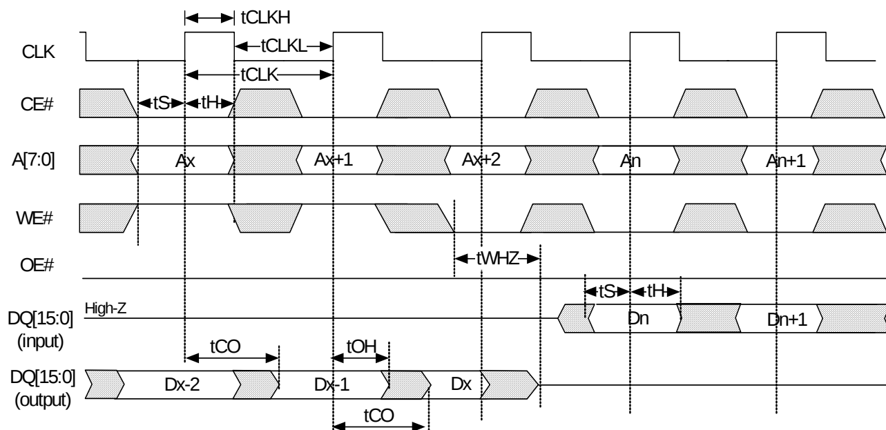
Figure 14. Synchronous Read to Write (OE# Fixed LOW) Timing
