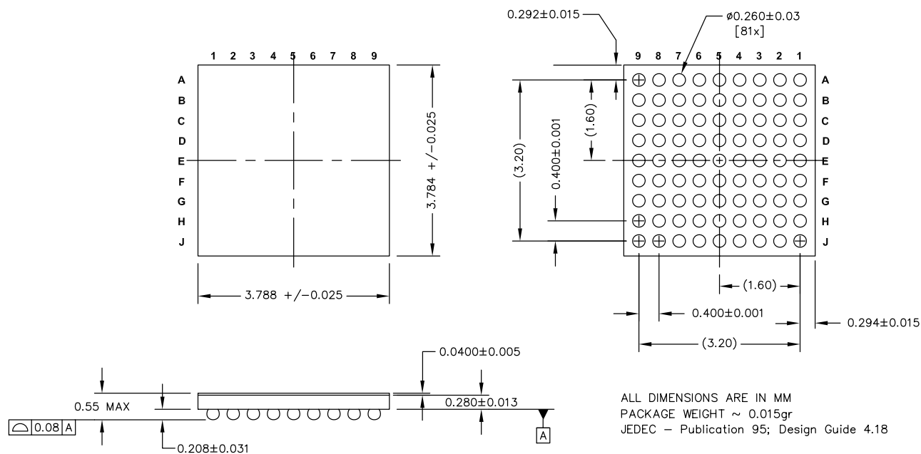
Figure 20. 81 WLCSP (3.784 × 3.788 × 0.55 mm)
