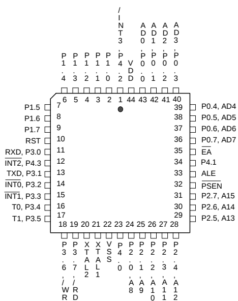
44-Pin PLCC
