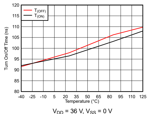
Figure 6-22. T_{\text{ON}} and T_{\text{OFF}} vs Temperature
