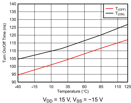
Figure 6-21. T_{\text{ON}} and T_{\text{OFF}} vs Temperature
