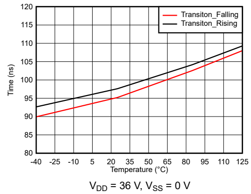
Figure 6-20. T_{\text{TRANSITION}} vs Temperature
