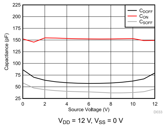
Figure 6-31. Capacitance vs Source Voltage or Drain Voltage
