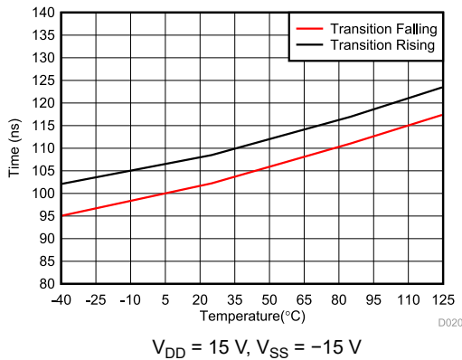
Figure 6-19. T_{\text{TRANSITION}} vs Temperature
