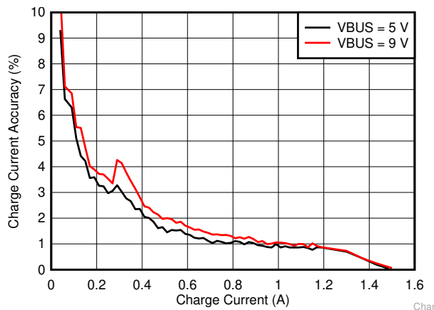
Figure 8-3. Charge Current Accuracy
