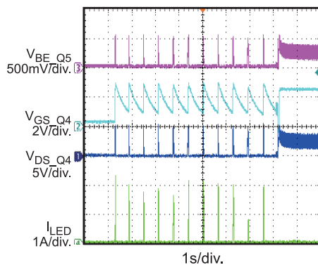
LED+ Short to LED- before Start-up then Recovery
