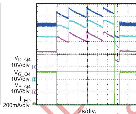
Output Open at Normal Operation then Recovery
