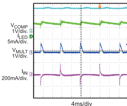
Triac Dimming
