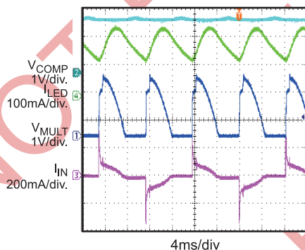
Triac Dimming
