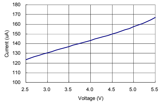
AIVIN Shutdown Current vs AVIN
