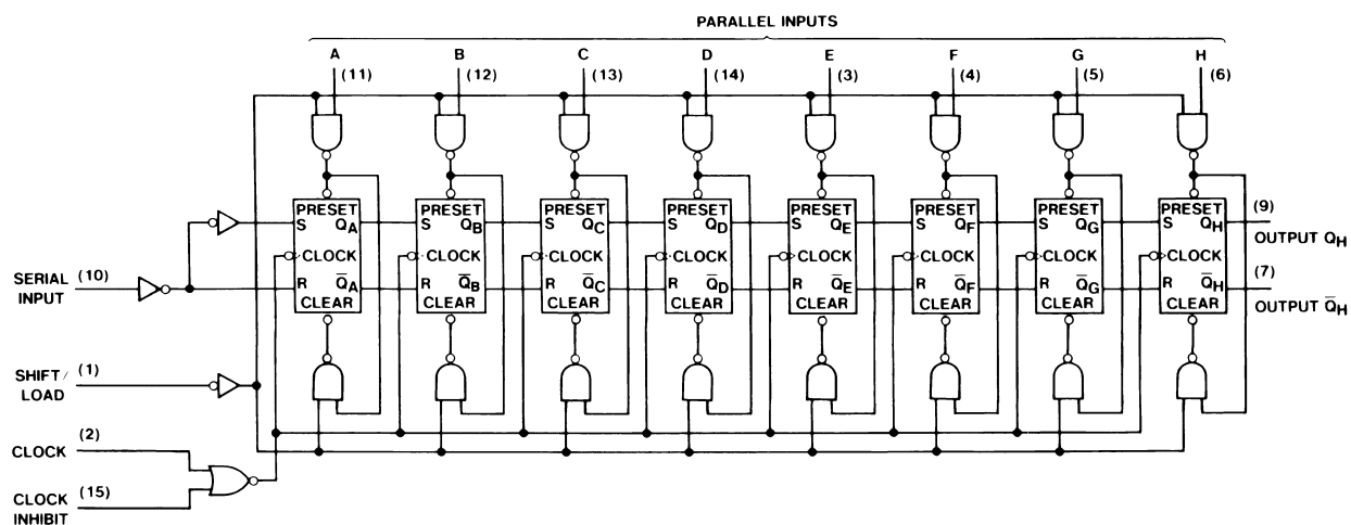
Logic Diagram
