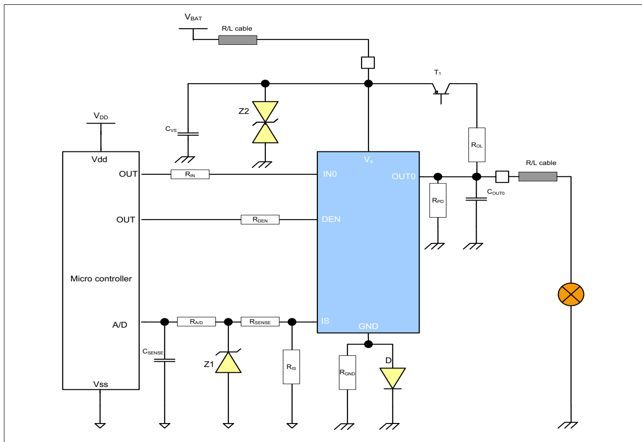
Figure 52 Application Diagram with BTS5012-1EKA
