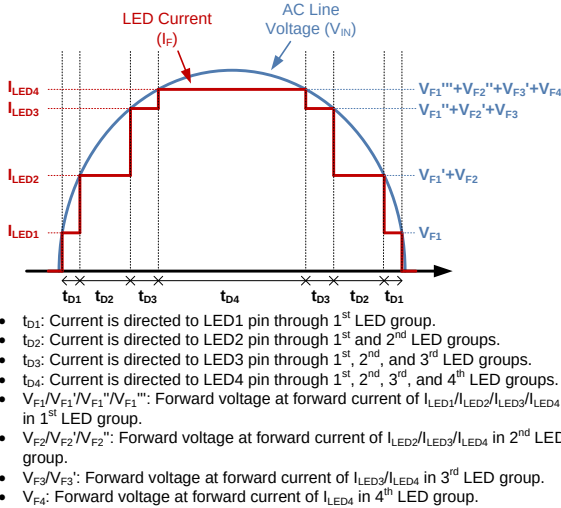
Figure 10. FL77904 Operation
