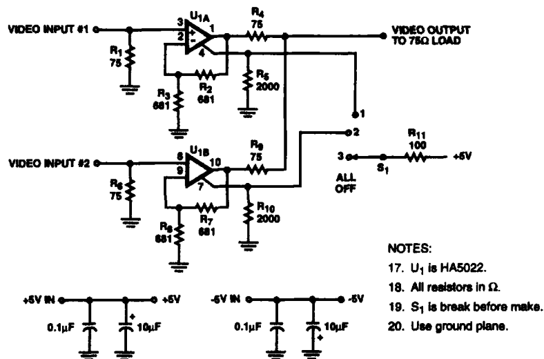
FIGURE 9. TWO CHANNEL HIGH IMPEDANCE MULTIPLEXER
