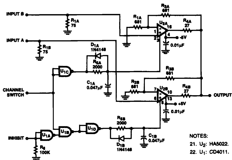
FIGURE 10. LOW IMPEDANCE MULTIPLEXER
