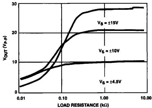
FIGURE 37. OUTPUT SWING vs LOAD RESISTANCE
