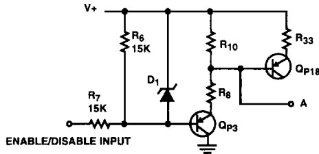
FIGURE 8. SIMPLIFIED SCHEMATIC OF ENABLE/DISABLE FUNCTION
