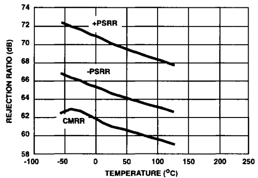
FIGURE 34. REJECTION RATIO vs TEMPERATURE
