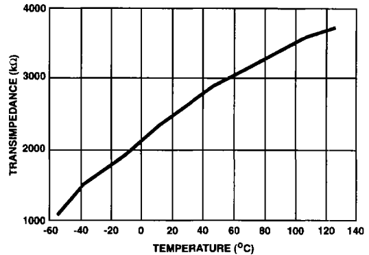
FIGURE 32. TRANSIMPEDANCE vs TEMPERATURE
