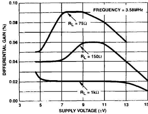
FIGURE 19. DIFFERENTIAL GAIN vs SUPPLY VOLTAGE
