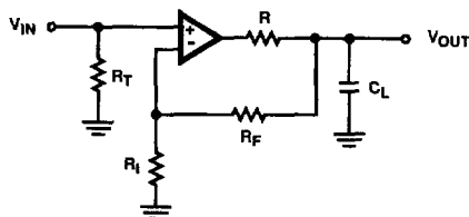
FIGURE 6. PLACEMENT OF THE OUTPUT ISOLATION RESISTOR, R
