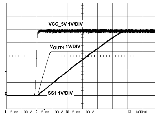
FIGURE 13. SOFT-START OPERATION
