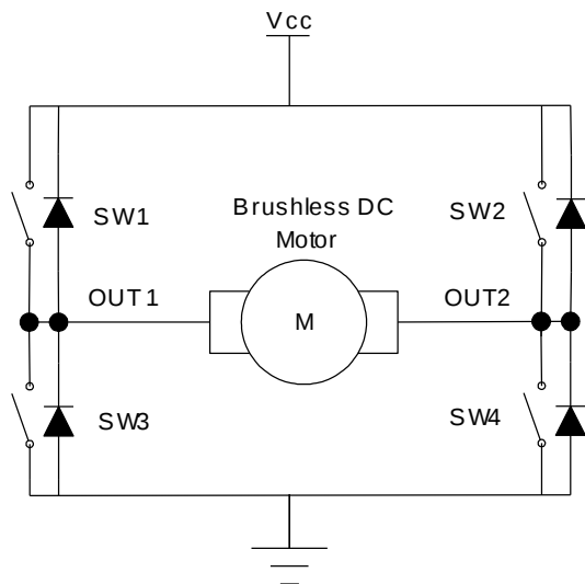
Figure 3: Power Stage
