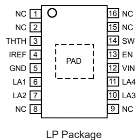
LP Package
