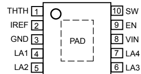
LY Package
