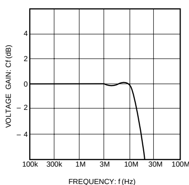
Fig. 3 Frequency characteristics
