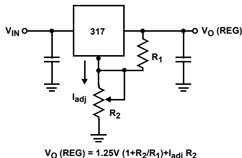
VOLTAGE REGULATOR
