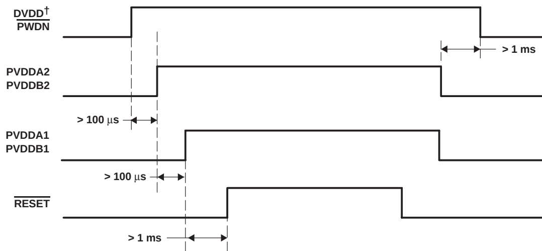
Figure 3. Power-Up/Power-Down Sequence
