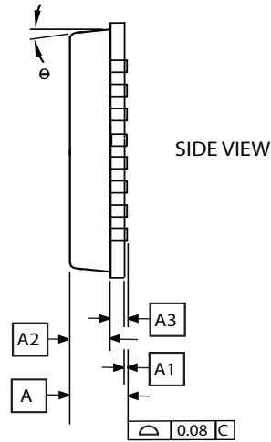
COMMON DIMENSIONS (Unit of Measure = mm)
