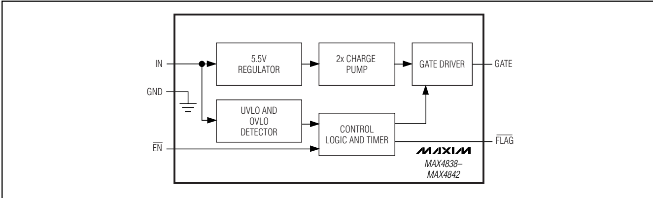
Figure 5. Functional Diagram
