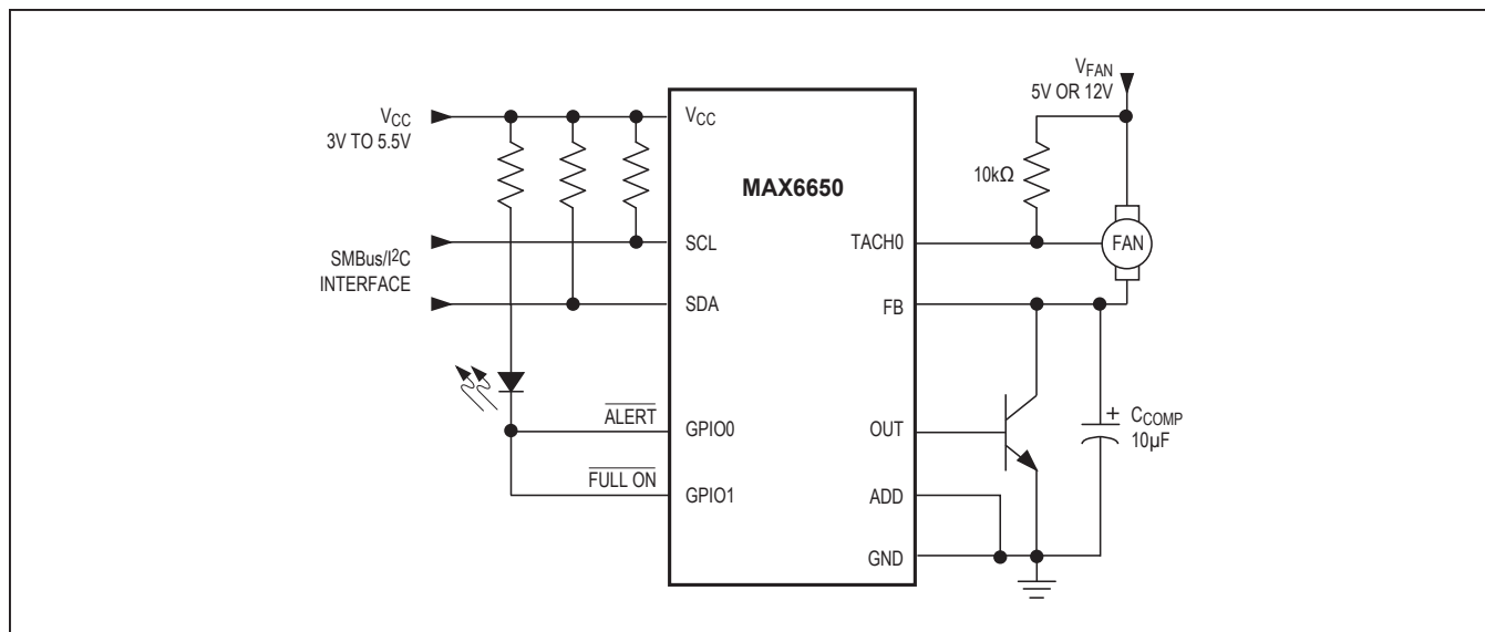
Figure 6. Fan Control with a Bipolar Transistor
