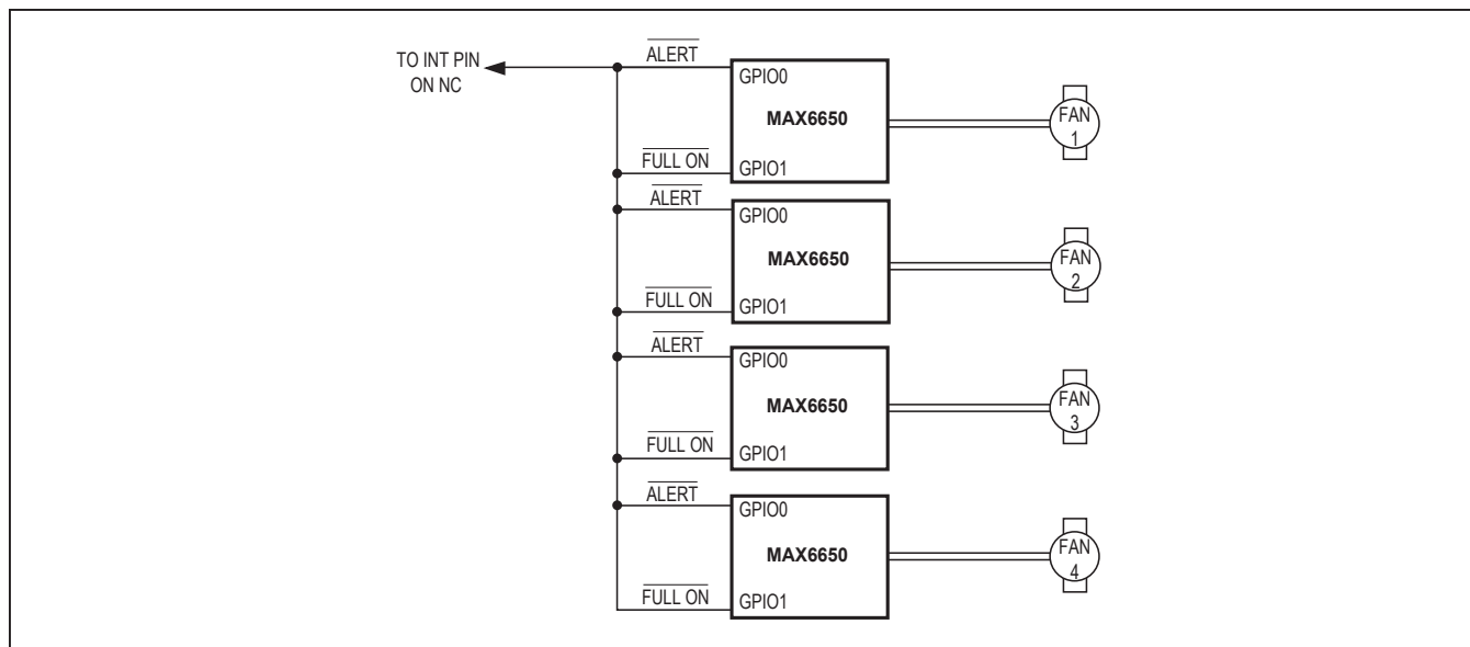
Figure 9. N + 1 Application
