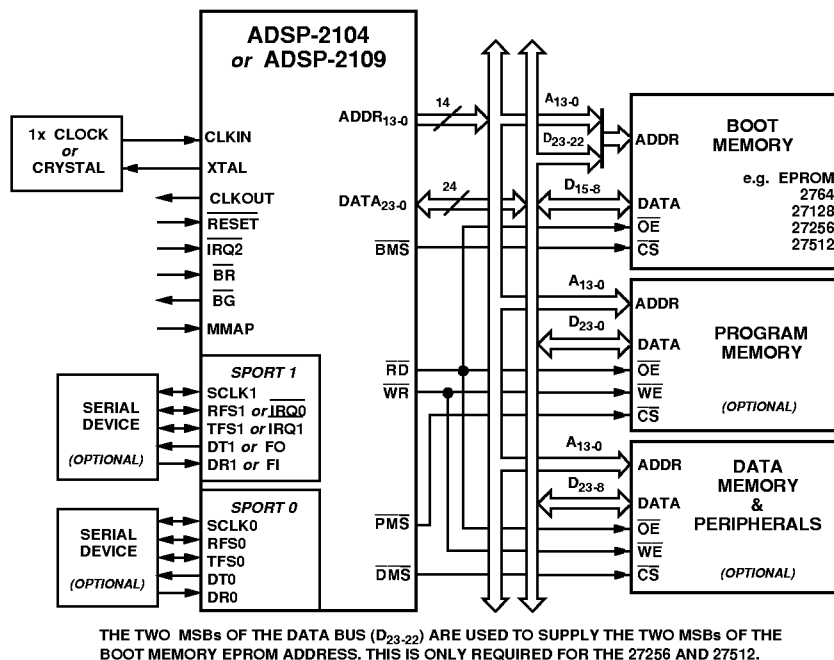
Figure 3. ADSP-2104/ADSP-2109 System
