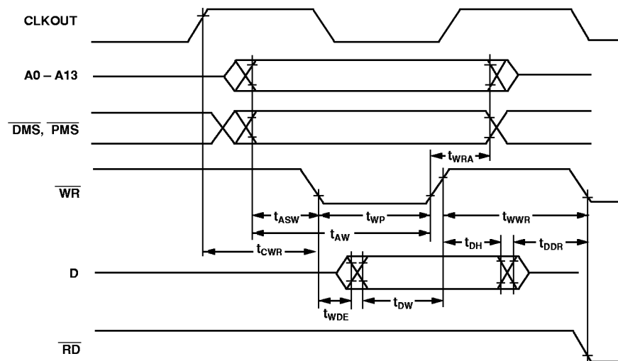
Figure 23. Memory Write
