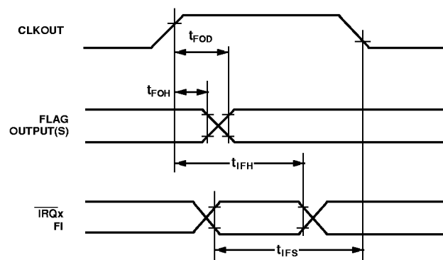
Figure 20. Interrupts & Flags
