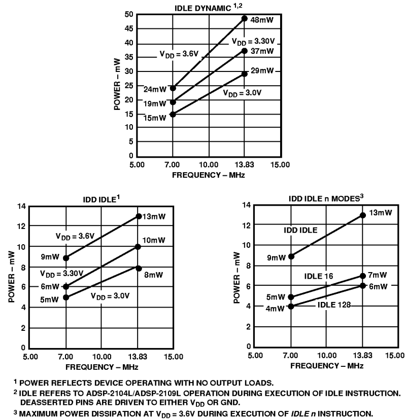
Figure 13. ADSP-2104L/ADSP-2109L Power (Typical) vs. Frequency
