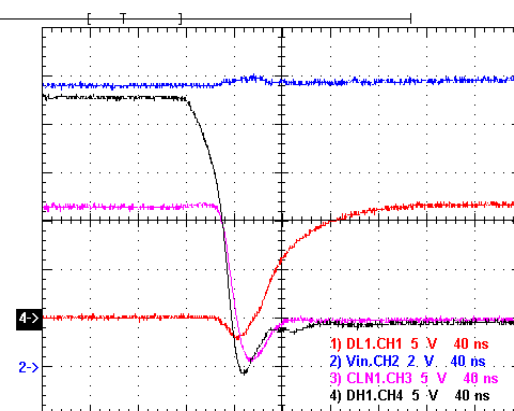
Figure 24. Dead Time at 18A Load (Falling Edge)
