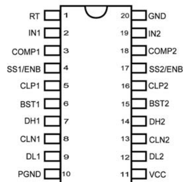
Figure 5. Pin Assignments (Top View)
