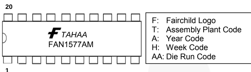
Figure 3. Marking Diagram
