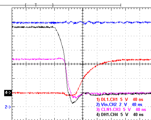
Figure 22. Dead Time at 0.3A Load (Falling Edge)
