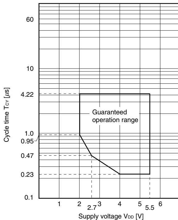
T_{CY} vs. V_{DD} (High-speed internal oscillator Clock)
