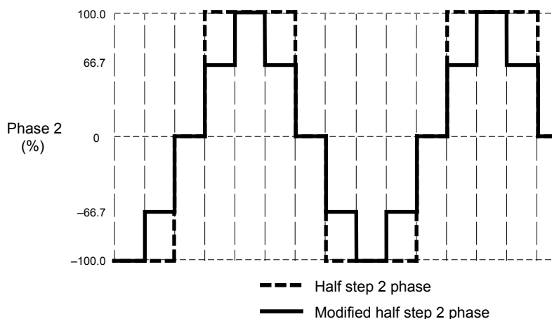
Figure 4: Step Sequencing for Half-Step Increments
