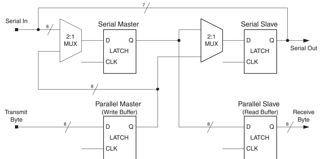
Figure 19-2. SPI Shift Register Diagram
