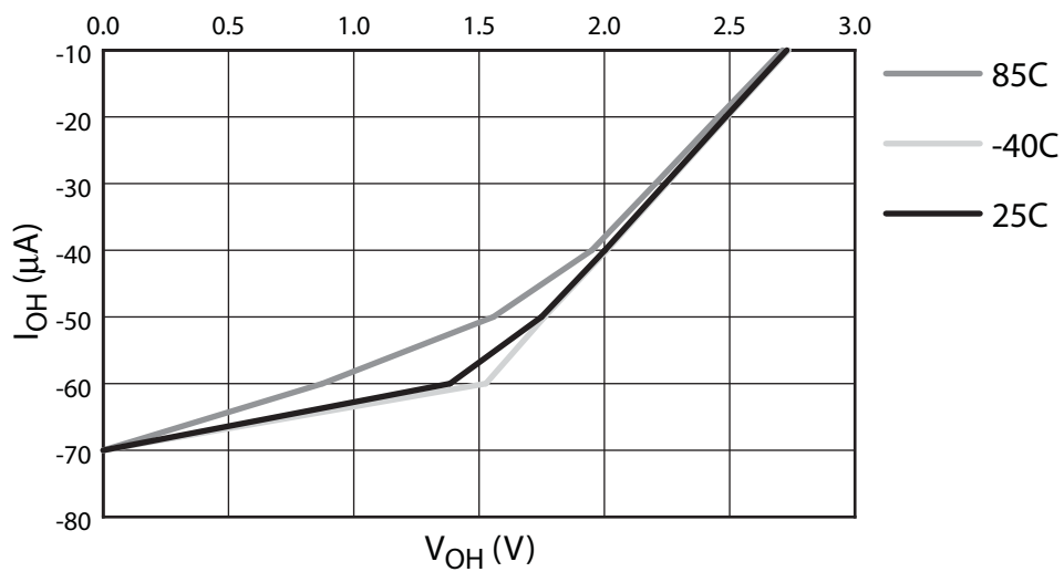
Figure 25-7. Quasi-Bidirectional Output I-V Characteristic at 3V
