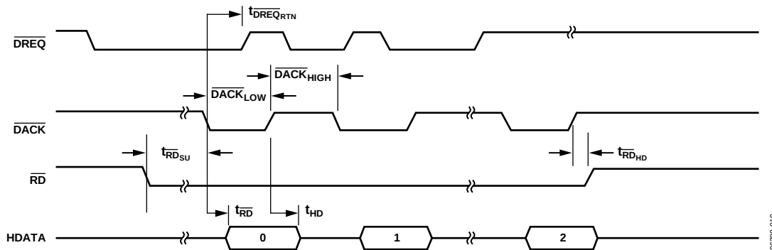
Figure 10. Single Read for \overline{\text{DREQ}}/\overline{\text{DACK}} DMA Mode for Assigned DMA Channel (EDMOD0/EDMOD1[14:11] Programmed to a Value of 0000)
