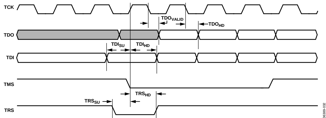
Figure 29. JTAG Timing
