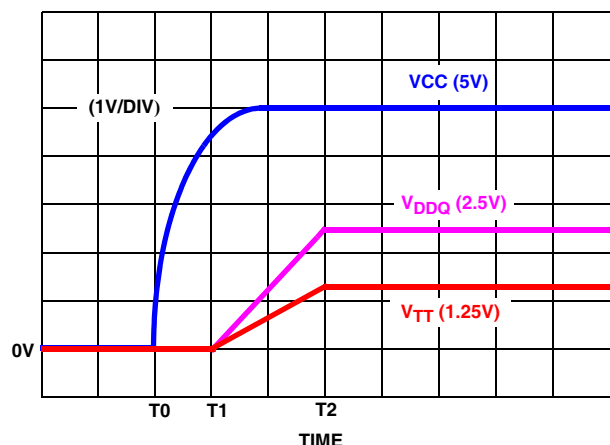
FIGURE 2. SOFT-START INTERVAL
