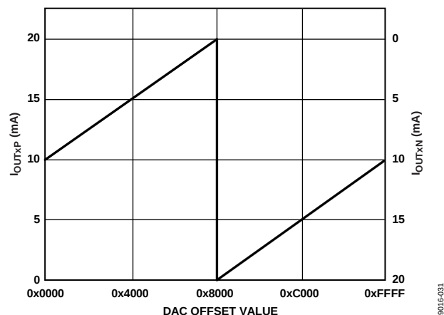
Figure 61. DAC Output Currents vs. DAC Offset Value
