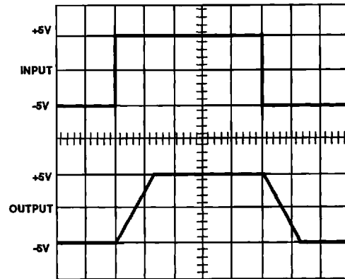
FIGURE 11. SLEW RESPONSE (Volts: 5V/Div., Time: 5 \mu s/Div.)
