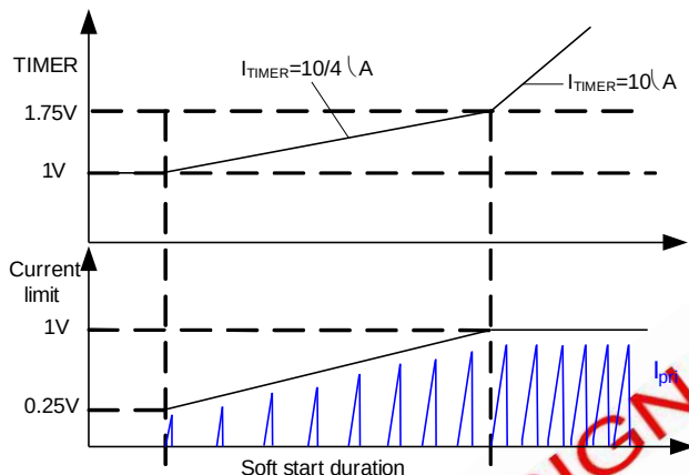
Figure 6: Soft-Start
