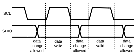
Figure 10. Data Validity Diagram
