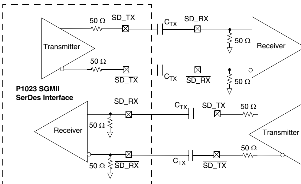
Figure 19. 4-Wire AC-Coupled SGMII Serial Link Connection Example
