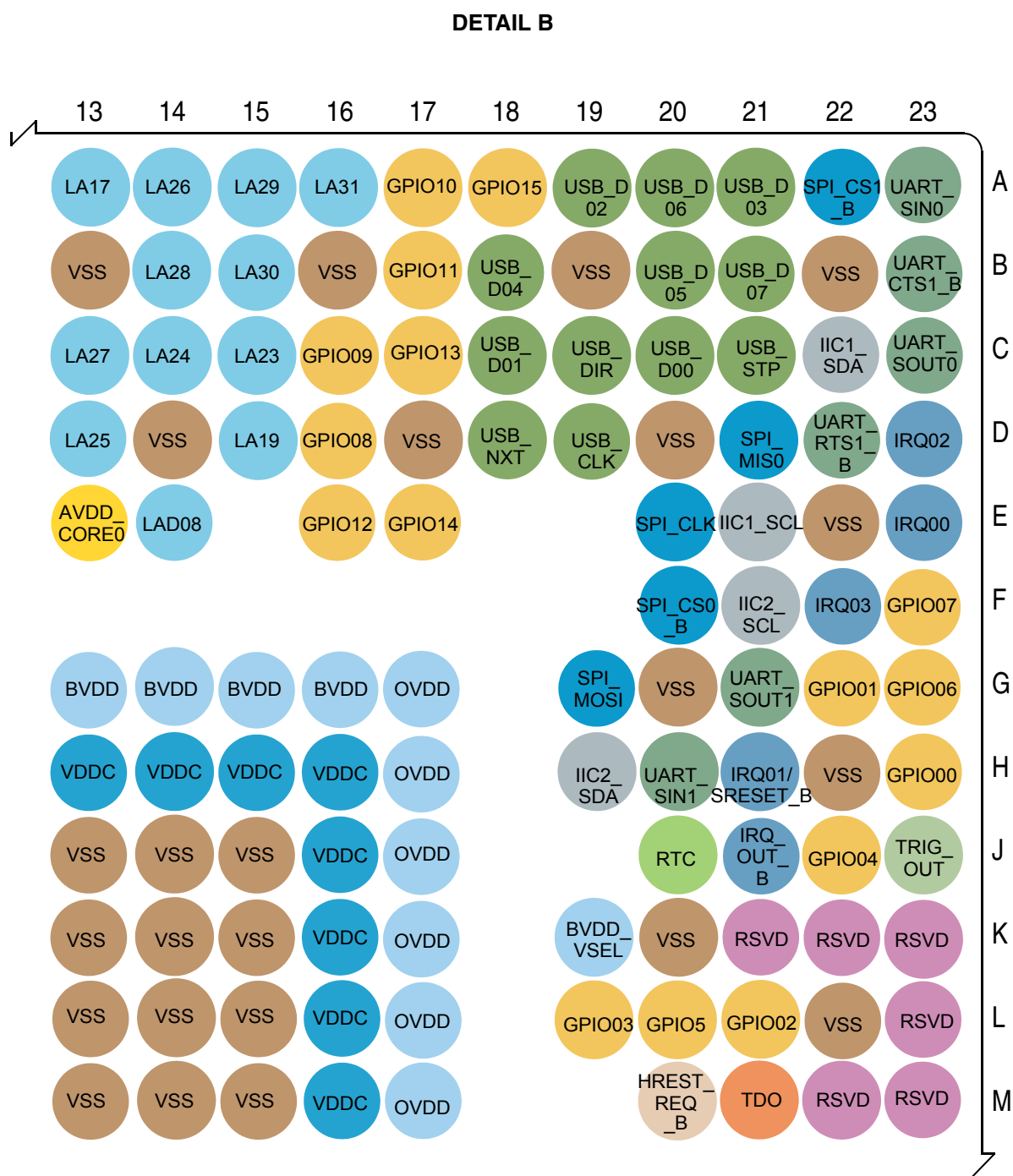
Figure 4. Ball Map—Detail B
