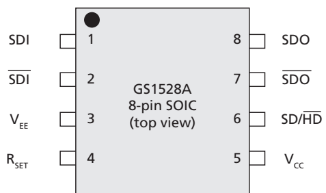
Figure 1-1: 8 Pin SOIC
