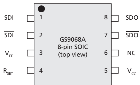
Figure 1-2: 8 Pin SOIC
