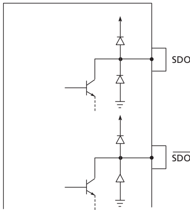
Figure 5-3: Static Protection Diodes
