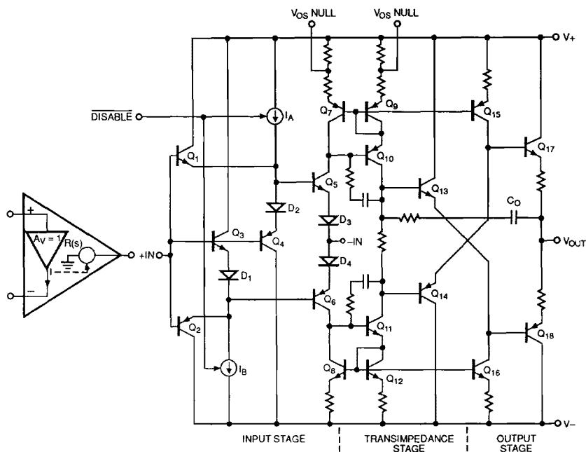
FIGURE 5: Simplified schematic of the OP-160 showing the three stages of the amplifier.
