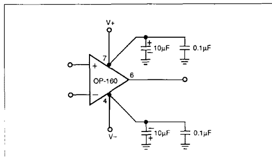
FIGURE 9: Proper power supply bypassing is required to obtain optimum performance with the OP-160.
