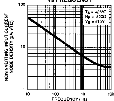
NONINVERTING INPUT CURRENT NOISE DENSITY vs FREQUENCY
