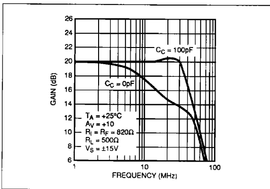
FIGURE 28: Gain/frequency graph for the compensated amplifier, A_V = +10 , showing the effect of the compensation capacitance, C_C , on gain flatness.
