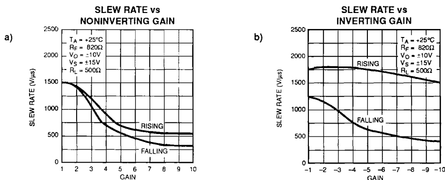
FIGURE 6: Slew rate of the OP-160 in noninverting (a) and inverting (b) configurations.
