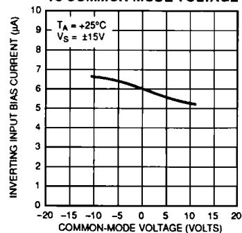
INVERTING INPUT BIAS CURRENT vs COMMON-MODE VOLTAGE
