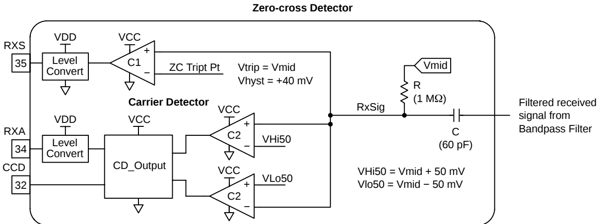
Figure 10. Receive Signal Detectors
