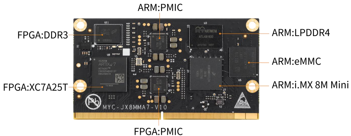
MYC-JX8MMA7 CPU Module Top-view
