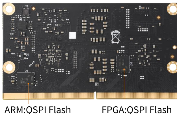
MYC-JX8MMA7 CPU Module Bottom-view
