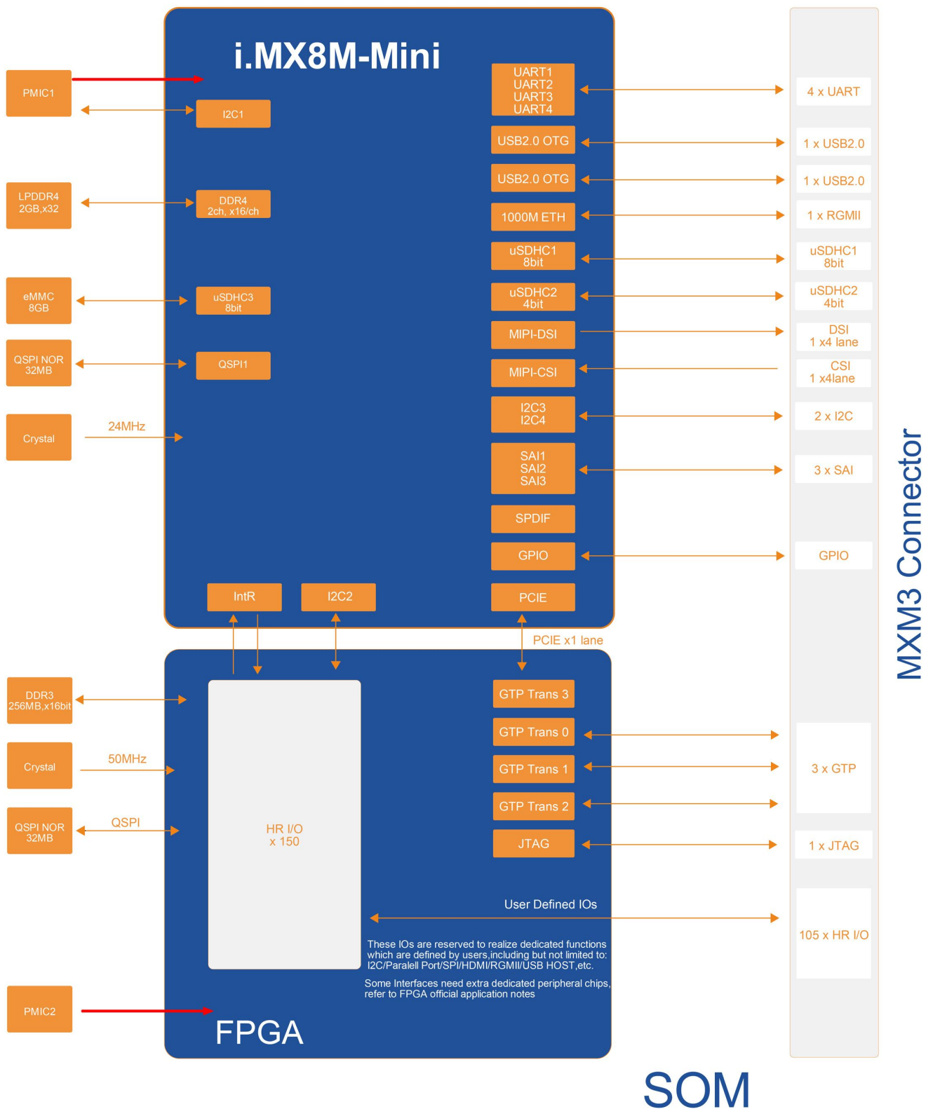
MYC-JX8MMA7 CPU Module Block Diagram
