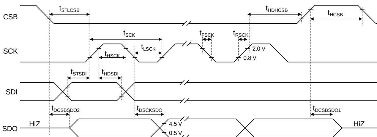
Figure 6. SPI Timing Chart
